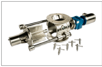
KLEAN-IN-PLACE II ROTARY VALVES
